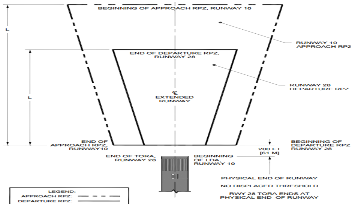
Exhibit 4-2 – FAA Runway Protection Zone
